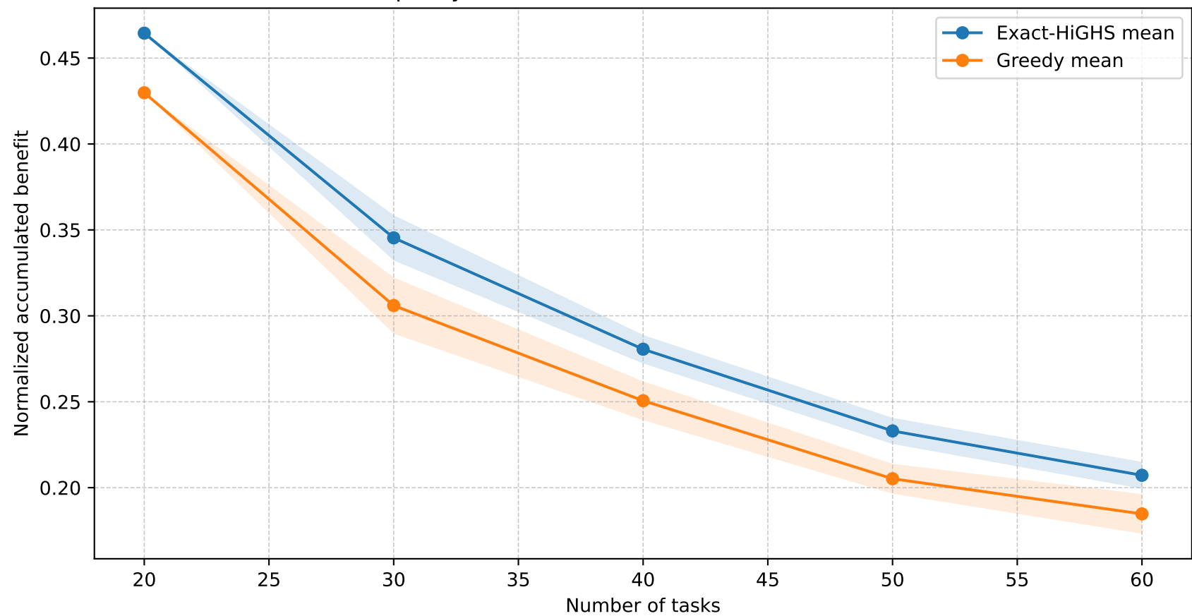
Solution quality across scaled TTAP instances - 4 areas / 4 helo
